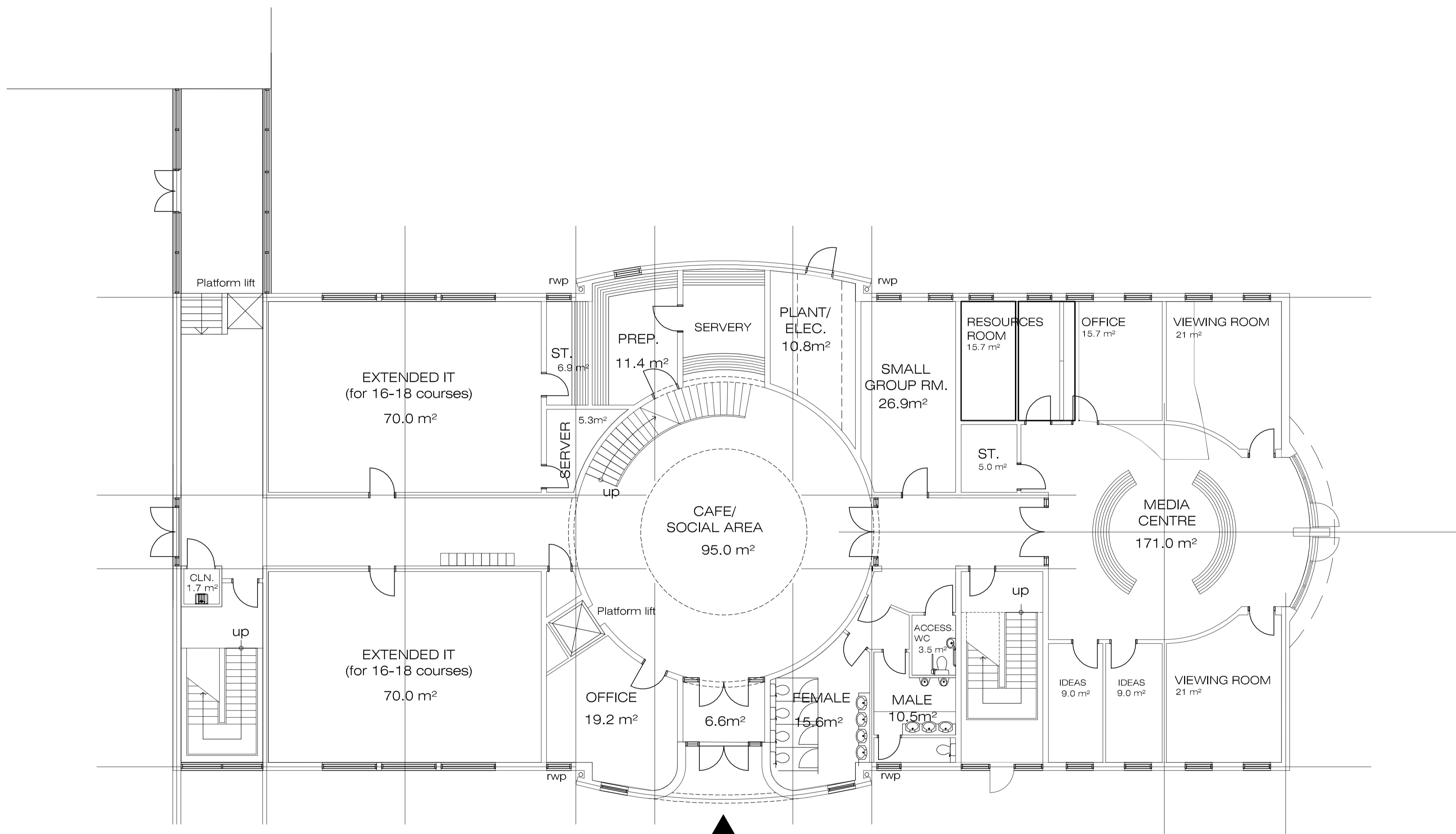
GROUND FLOOR PLAN 1:200 GIA = 722 m 2
